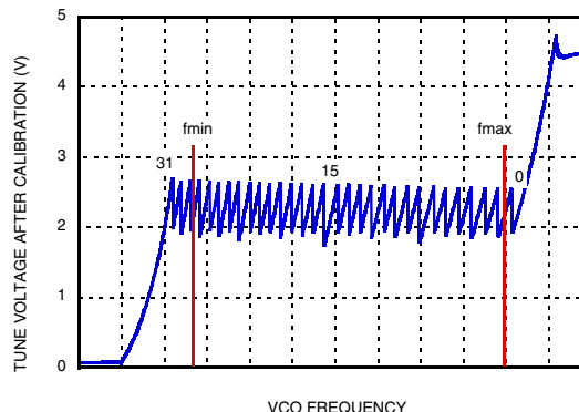
Figure 6. Typical Tuning Voltage After Calibration
