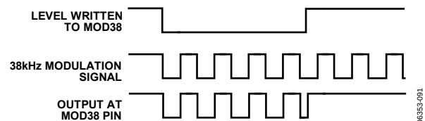
Figure 117. 38 kHz Modulation
