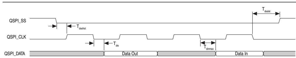
Figure 7. QSPI Timing Diagram
