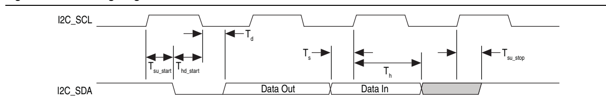
Figure 15. I 2 C Timing Diagram
