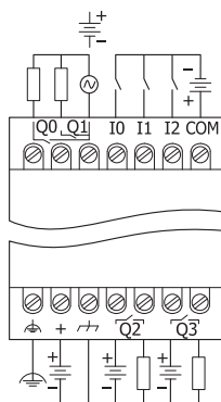
Connection diagram
