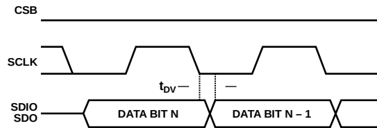
Figure 56. Timing Diagram for Serial Control Port Register Read
