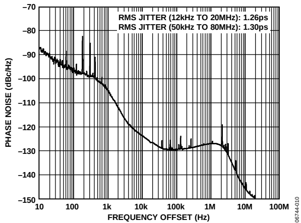
Figure 10. Additive Phase Noise at HSTL Output Driver, SYSCCLK = 1\text{ GHz} ( SYSCCLK PLL Enabled and Driven by a 25 MHz Fox Crystal Oscillator), f_{REF} = 19.44\text{ MHz} , f_{OUT} = 155.52\text{ MHz} , DPLL Loop BW = 1 kHz
