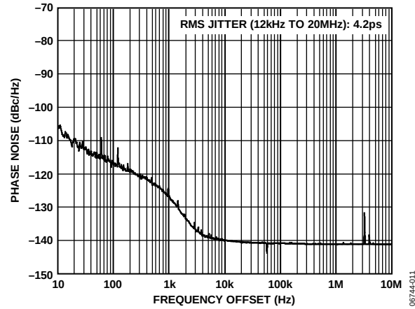
Figure 11. Additive Phase Noise at HSTL Output Driver, SYSCCLK = 500\text{ MHz} ( SYSCCLK PLL Disabled), f_{REF} = 10.24\text{ MHz} , f_{OUT} = 20.48\text{ MHz} , DPLL Loop BW = 1 kHz
