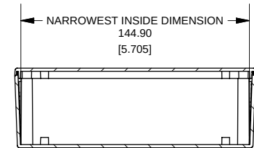
SECTION C-C
