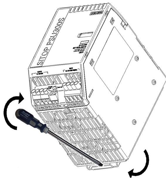
Bild 2: Montage Figure 2: Mounting Figure 2: Fixation Figura 2: Montaggio Figura 2: Montaje
