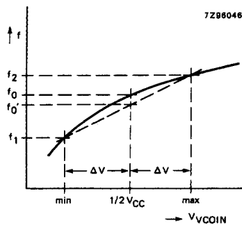
Fig.20 Definition of VCO frequency linearity: \Delta V = 0.5 \text{ V} over the V_{CC} range: for VCO linearity
