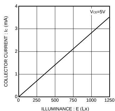
Fig.1 Collector current-Illuminance
