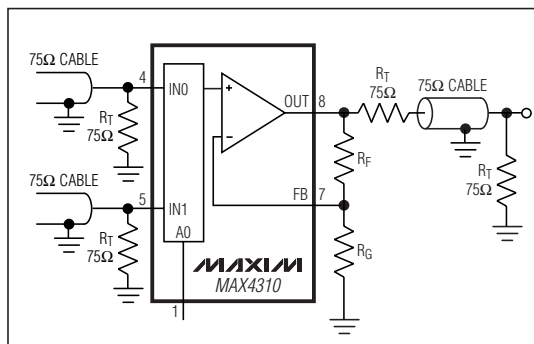
Figure 1. MAX4310 Noninverting Gain Configuration
