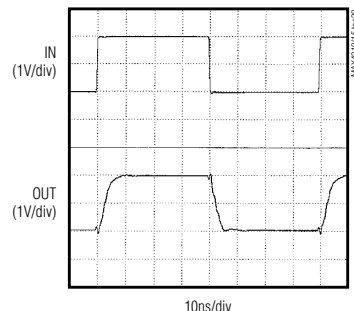
MAX4310 LARGE-SIGNAL PULSE RESPONSE
