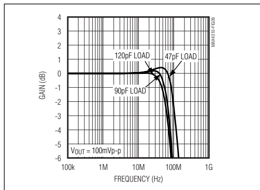
Figure 9. Small-Signal Gain vs. Frequency with a Capacitive Load and 27Ω No-Isolation Resistor
