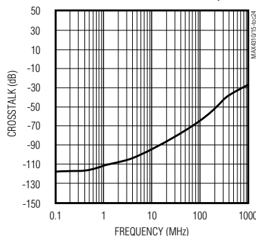
MAX4310/MAX4313 ALL-HOSTILE CROSSTALK vs. FREQUENCY
