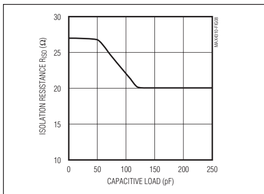
Figure 8. Optimal Isolation Resistance vs. Capacitive Load
