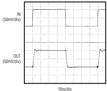
MAX4310 SMALL-SIGNAL PULSE RESPONSE
