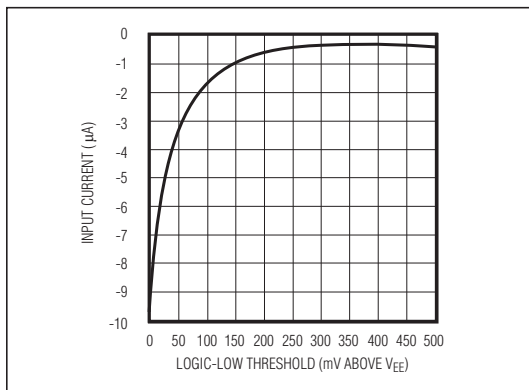
Figure 4. Logic-Low Input Current vs. V_{IL} with 10k \Omega Series Resistor
