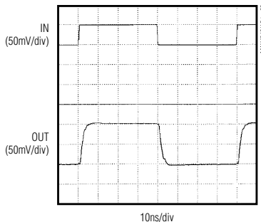
MAX4313 SMALL-SIGNAL PULSE RESPONSE
