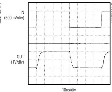
MAX4313 LARGE-SIGNAL PULSE RESPONSE
