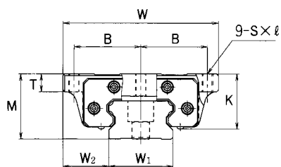
HSR-HA Type
