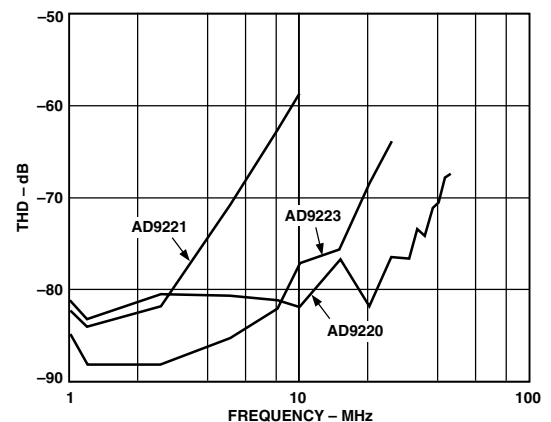
Figure 17. AD9221/AD9223/AD9220 THD vs. Input Frequency ( V_{\text{CM}} = 2.5\text{ V} , 2 V p-p Input Span, A_{\text{IN}} = -0.5\text{ dB} )
