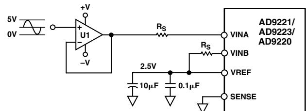
Figure 13. Single-Ended AD9221/AD9223/AD9220 Op Amp Drive Circuit
