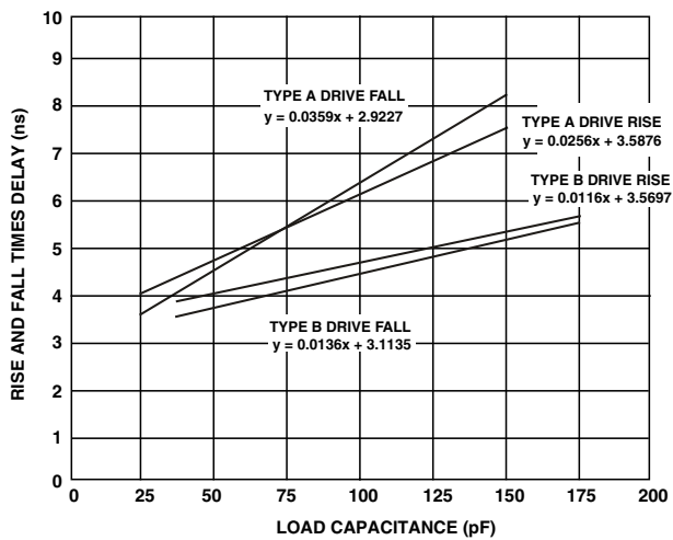
Figure 53. Typical Output Rise/Fall Delay Non-DDR ( V_{DD\_EXT} = \text{Min} )
