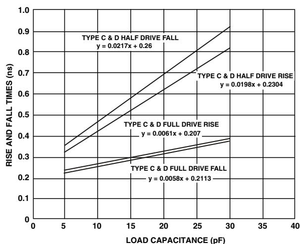
Figure 51. Typical Output Rise/Fall Time DDR2 (20% to 80%, V_{DD\_EXT} = \text{Max} )
