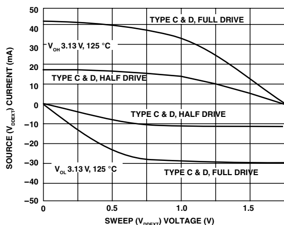
Figure 48. Output Buffer Characteristics (Worst-Case DDR2)
