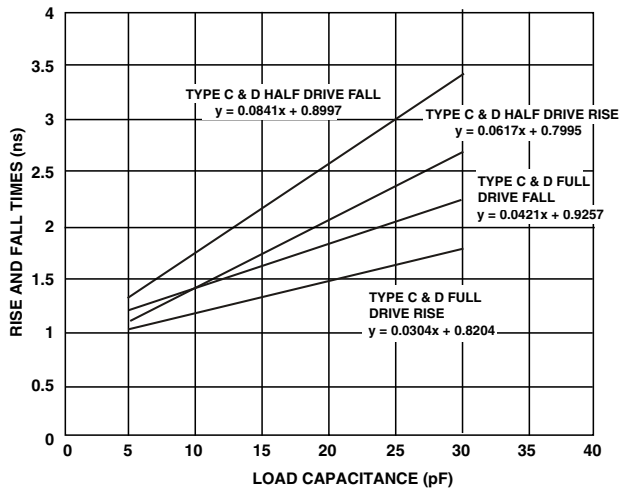
Figure 52. Typical Output Rise/Fall Time DDR2 (20% to 80%, V_{DD\_EXT} = \text{Min} )
