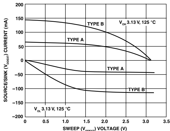
Figure 47. Output Buffer Characteristics (Worst-Case Non-DDR2)
