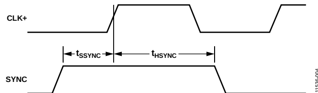
Figure 5. SYNC Input Timing Requirements
