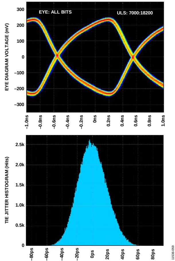
Figure 49. Data Eye for LVDS Outputs in ANSI-644 Mode with Trace Lengths of Greater Than 24 Inches on Standard FR-4 Material, External 100 \Omega Far End Termination Only
