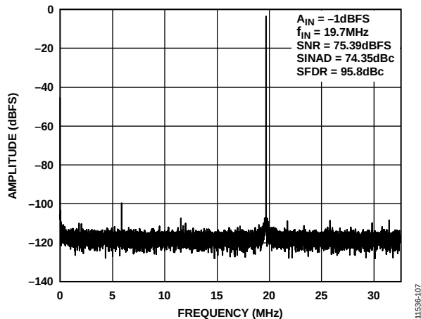
Figure 8. Single-Tone 32k FFT with f_{IN} = 19.7\text{ MHz} , f_{SAMPLE} = 65\text{ MSPS}
