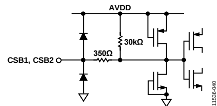
Figure 30. Equivalent CSBx Input Circuit
