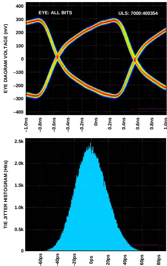
Figure 48. Data Eye for LVDS Outputs in ANSI-644 Mode with Trace Lengths of Less Than 24 Inches on Standard FR-4 Material, External 100 \Omega Far End Termination Only
