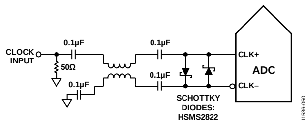
Figure 40. Balun-Coupled Differential Clock (65 MHz to 520 MHz)
