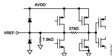
Figure 31. Equivalent VREF Circuit
