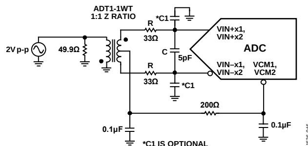
Figure 36. Differential Transformer Coupled Configuration for Baseband Applications
