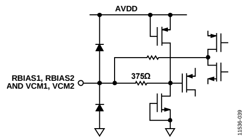
Figure 29. Equivalent RBIASx and VCMx Circuit
