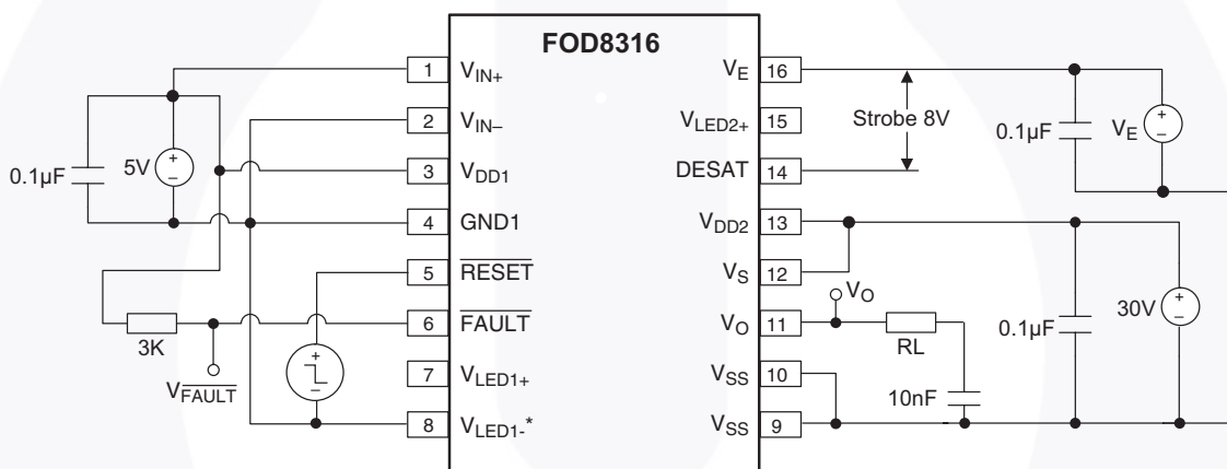
Figure 41. DESAT Sense ( t_{DESAT(90\%)} , t_{DESAT(10\%)} ), DESAT Fault ( t_{DESAT(FAULT)} ), and ( t_{DESAT(LOW)} ) Test Circuit
