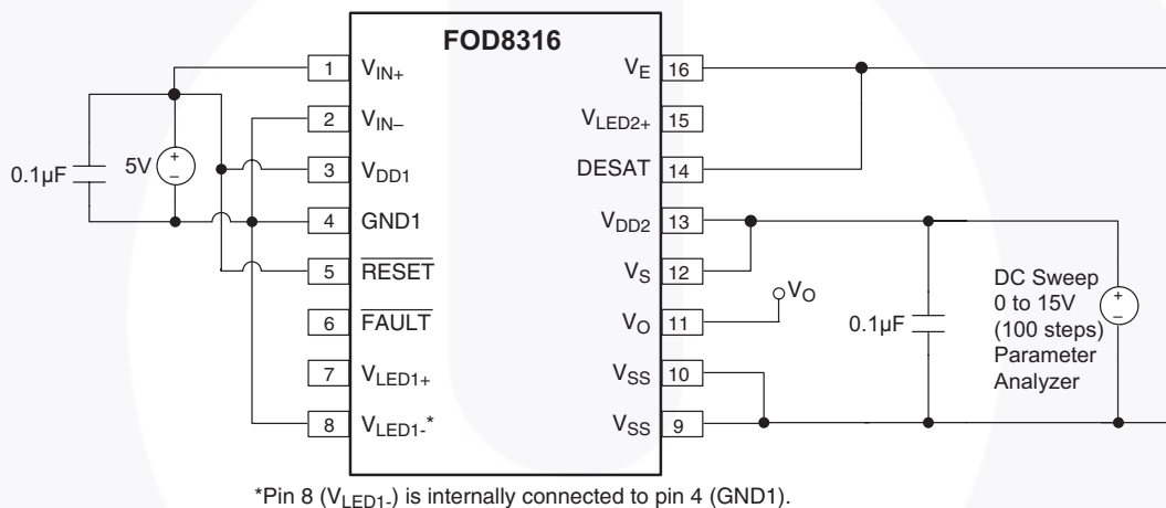
Figure 39. Under Voltage Lockout Threshold ( V_{UVLO} ) Test Circuit
