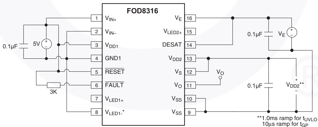
Figure 43. Under Voltage Lockout Delay ( t_{UVLO} ) and Time to Good Power ( t_{GP} ) Test Circuit
