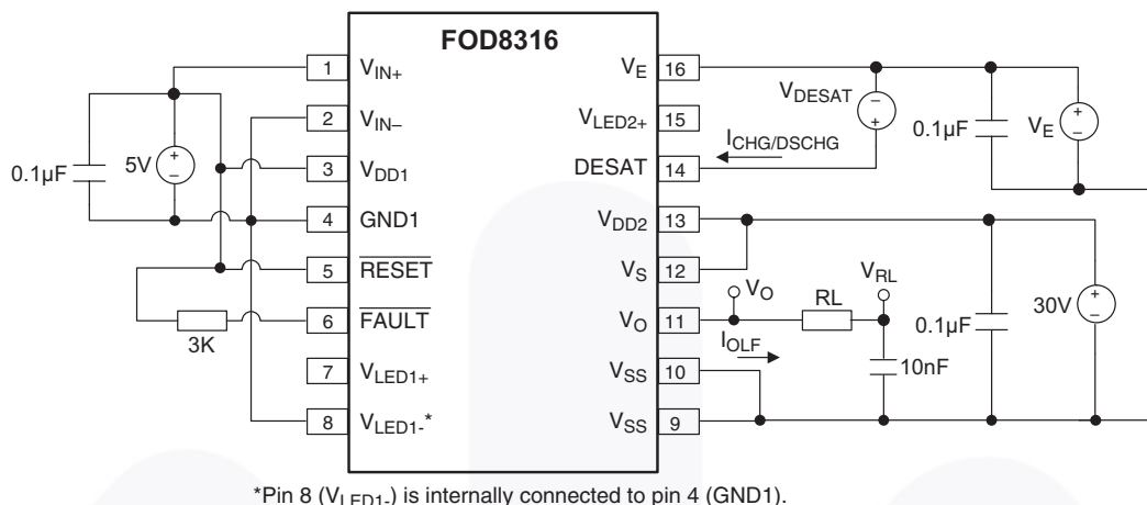
Figure 38. Low Level Output Current During Fault Conditions ( I_{OLF} ), Blanking Capacitor Charge Current ( I_{CHG} ), Blanking Capacitor Discharging Current ( I_{DSCHG} ) and DESAT Threshold ( V_{DESAT} ) Test Circuit
