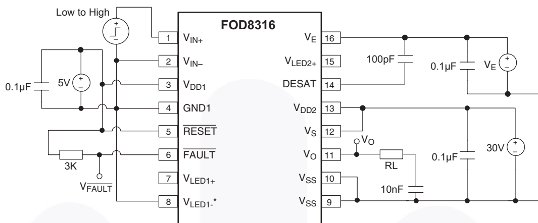
Figure 41. DESAT Sense ( t_{DESAT(90\%)} , t_{DESAT(10\%)} ), DESAT Fault ( t_{DESAT(FAULT)} ), and ( t_{DESAT(LOW)} ) Test Circuit
