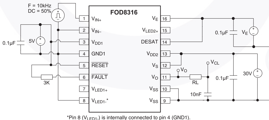
Figure 40. Propagation Delay ( t_{PLH} , t_{PHL} ), Pulse Width Distortion (PWD), Rise Time ( t_R ) and Fall Time ( t_F ) Test Circuit
