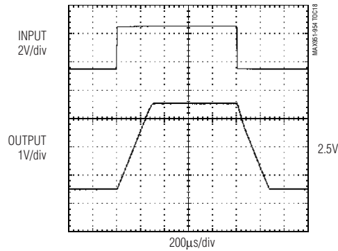
MAX951/MAX953 OP AMP LARGE-SIGNAL TRANSIENT RESPONSE
