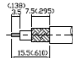
STRIPPING DIMENSION
