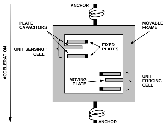
Figure 8. MEMS Sensor Diagram
