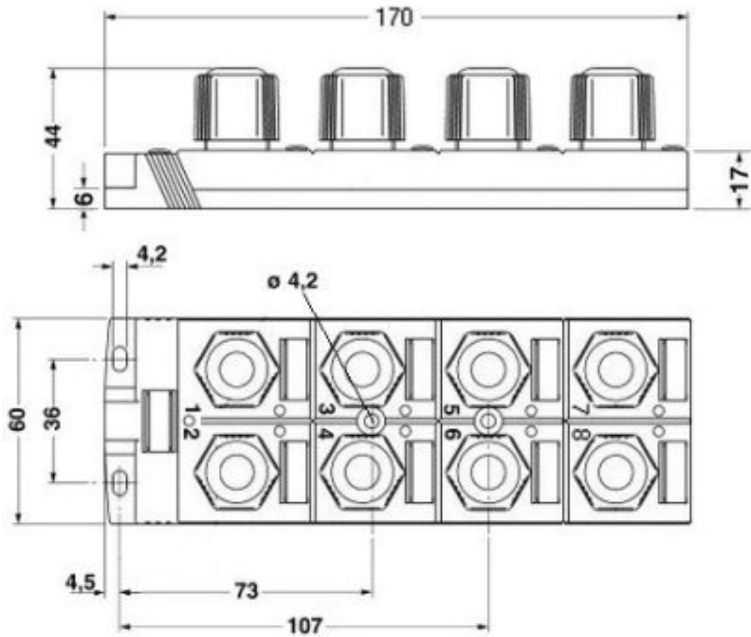
Dimensioned drawing
