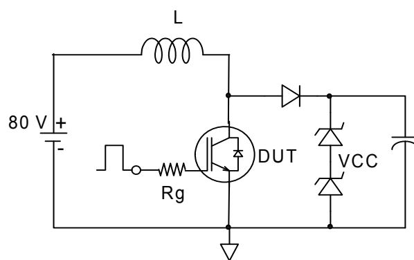
Fig.C.T.2 - RBSOA Circuit
