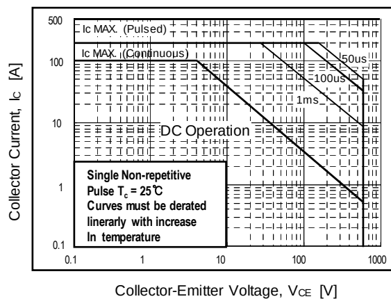
Fig14. SOA characteristics
