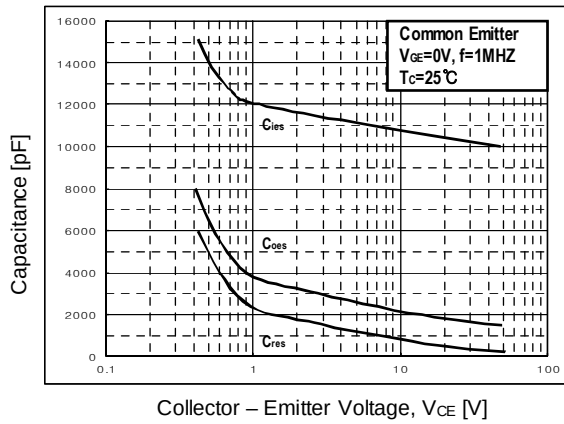
Fig 7. Capacitance characteristics
