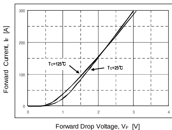
Fig 15. Forward characteristics
