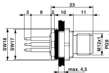
Dimensioned drawing
