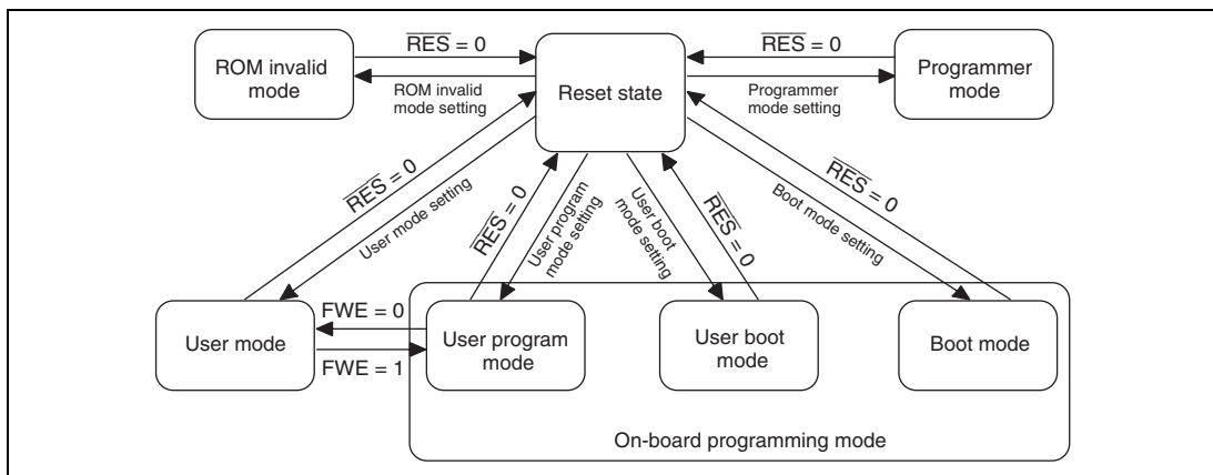
Figure 21.2 Mode Transition of Flash Memory
