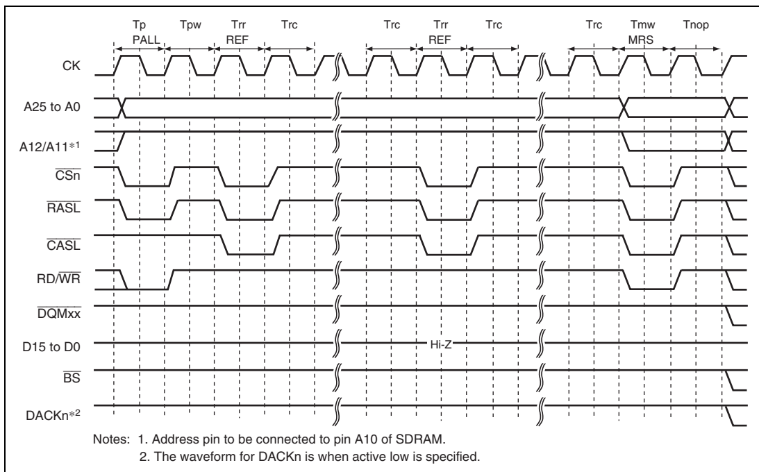
Figure 8.29 SDRAM Mode Write Timing (Based on JEDEC)
