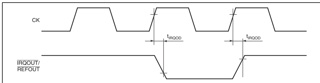
Figure 27.11 Bus Release Timing
