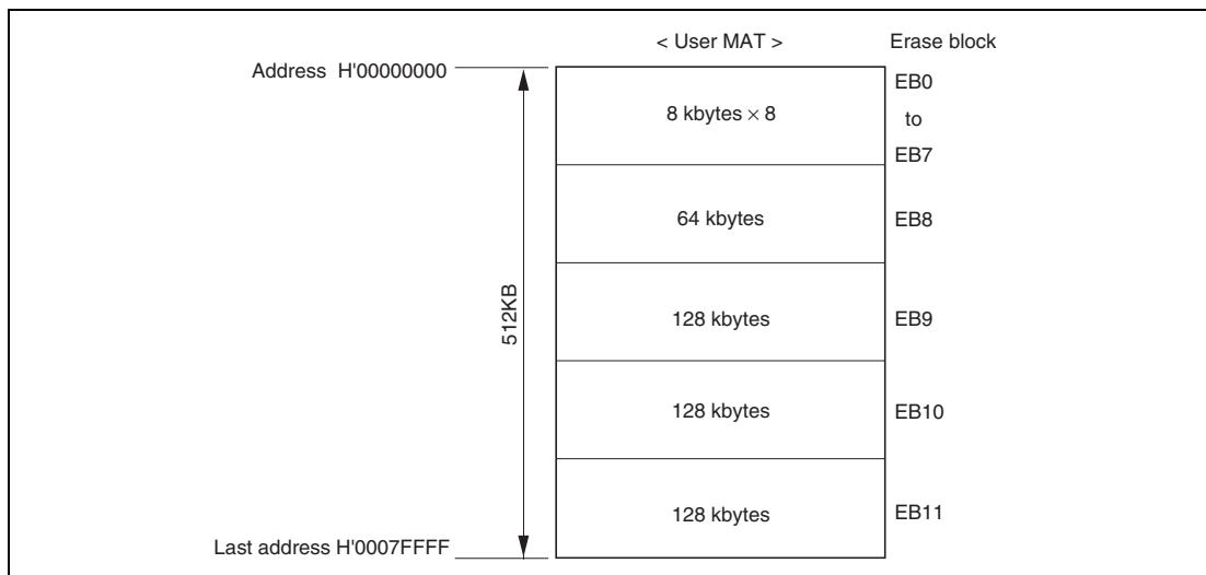
Figure 21.4 Block Division of User MAT
