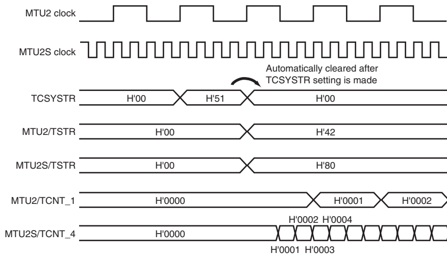
Figure 10.84 (4) Example of Synchronous Counter Start Operation (MTU2-to-MTU2S Clock Frequency Ratio = 1:4)
