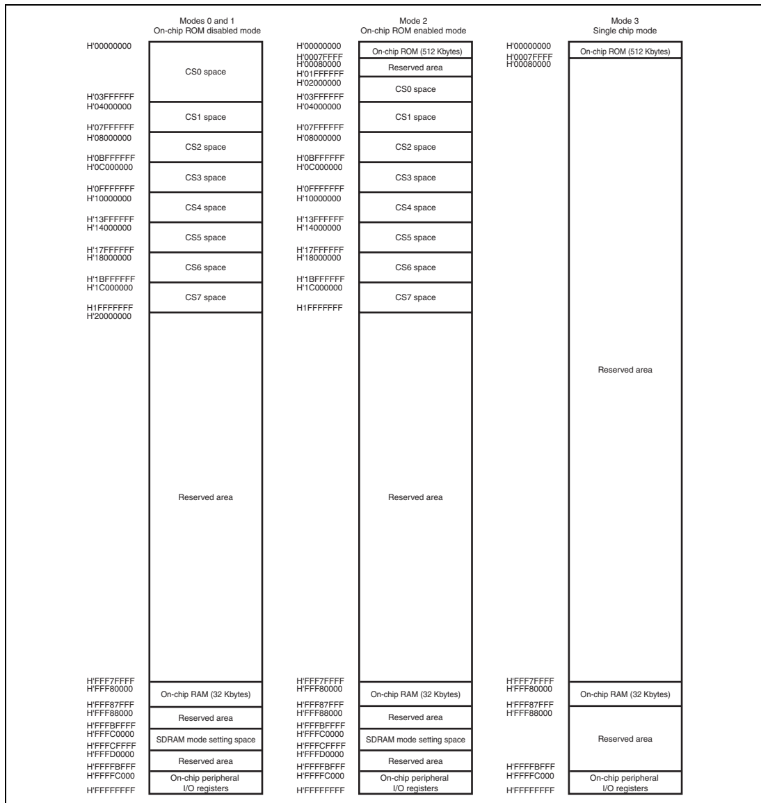
Figure 3.1 Address Map for Each Operating Mode
