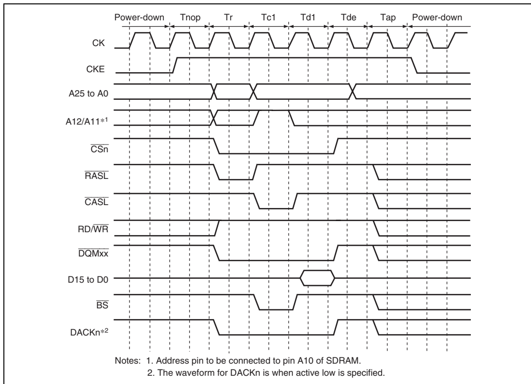
Figure 8.28 Power-Down Mode Access Timing
