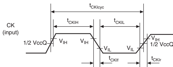
Figure 27.3 CK Clock Input Timing
