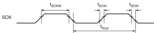
Figure 27.46 SCK Input Clock Timing
