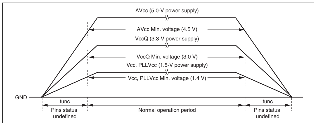
Figure 27.1 Power-on/Power-off Sequence
