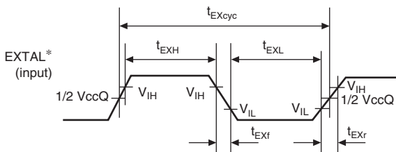
Figure 27.2 EXTAL Clock Input Timing
