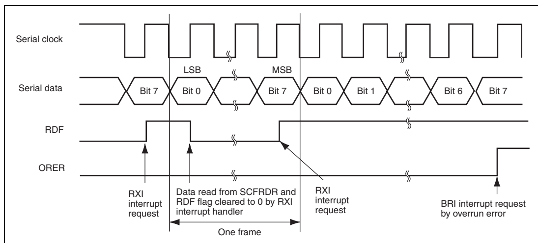
Figure 15.15 Example of SCIF Receive Operation
