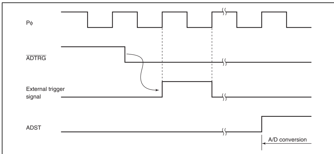
Figure 17.5 External Trigger Input Timing
