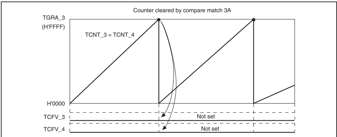
Figure 10.132 Reset Synchronous PWM Mode Overflow Flag
