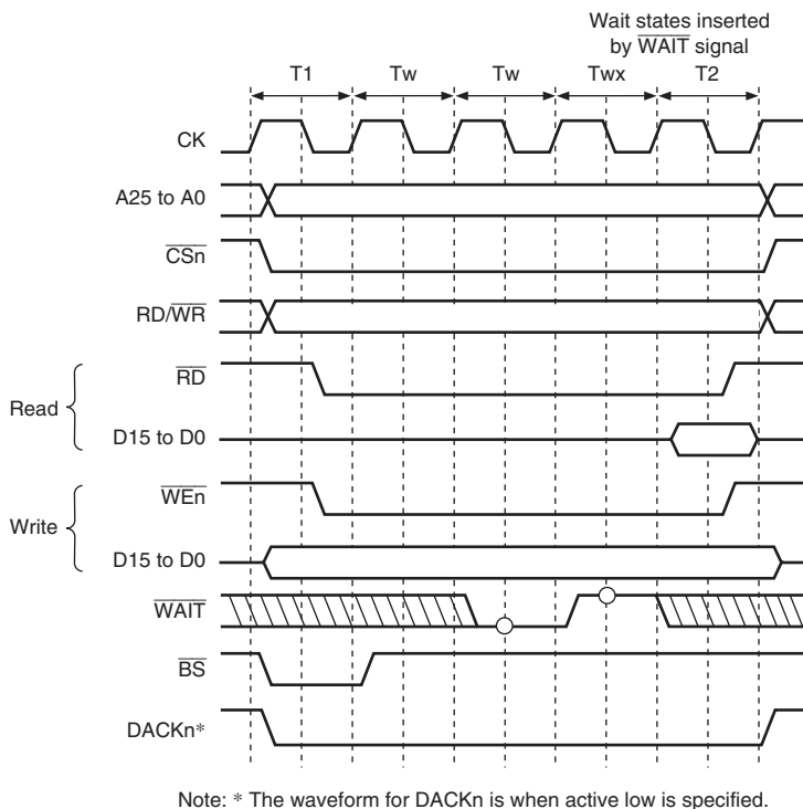
Figure 8.8 Wait Cycle Timing for Normal Space Access (Wait Cycle Insertion Using \overline{\text{WAIT}} Signal)
