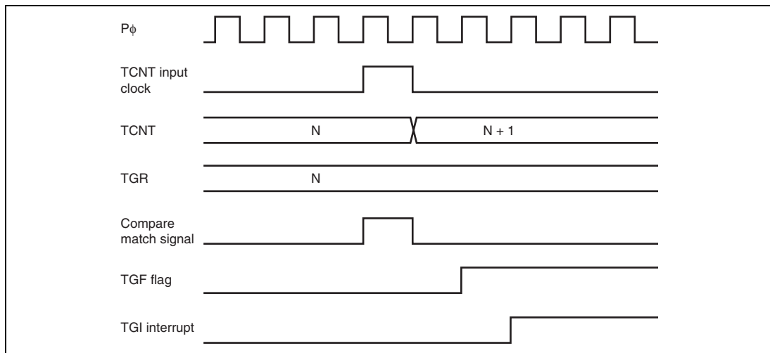
Figure 10.109 TGI Interrupt Timing (Compare Match)
