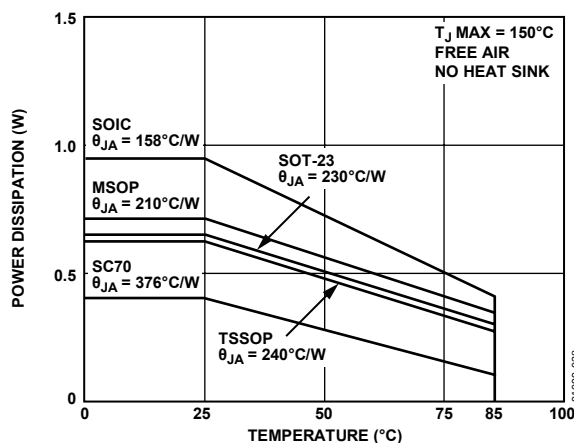
Figure 38. Maximum Power Dissipation vs. Ambient Temperature
