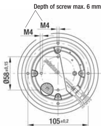
Depth of screw max. 6 mm
