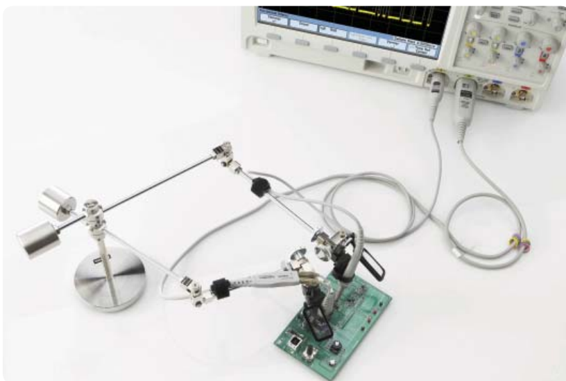
N2785A Two-arm probe positioner
