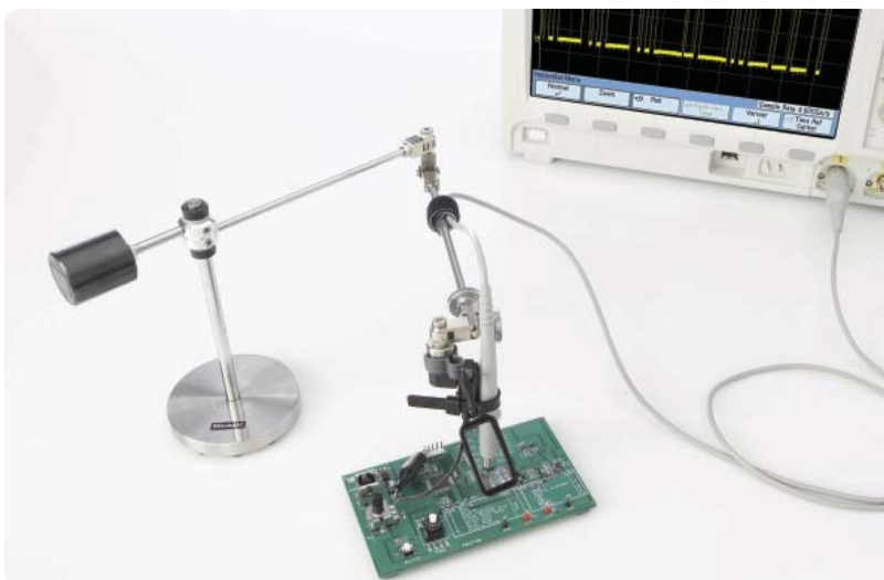
N2784A one-arm probe positioner
