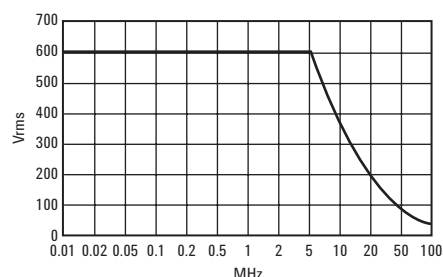
Derating of each input for the N2772A
