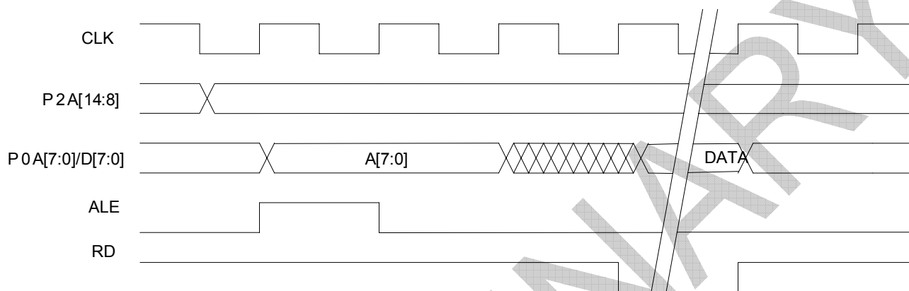
FIGURE 37: DATA MEMORY READ CYCLE TIMING
