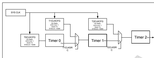
FIGURE 12: TIMER CHAINING
