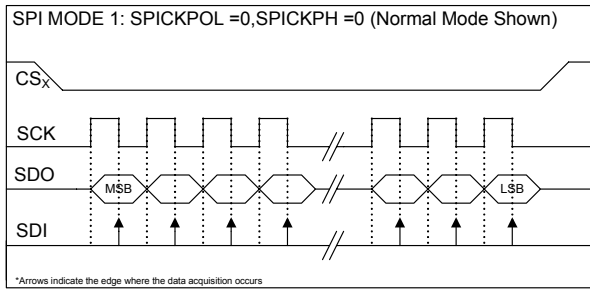
FIGURE 17: SPI MODE 1
