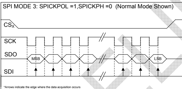
FIGURE 19: SPI MODE 3
