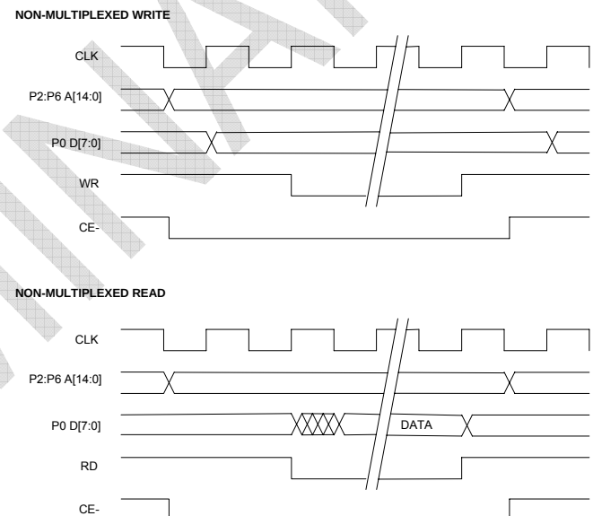
FIGURE 6: NON-MULTIPLEXED EXTERNAL DATA MEMORY ACCESS
