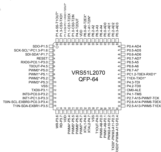
FIGURE 2: VRS51L2070 QFP-64 PIN OUT DIAGRAMS
