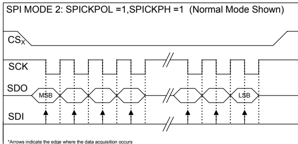
FIGURE 18: SPI MODE 2
