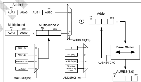
FIGURE 31: ARITHMETIC UNIT MULTIPLICATION AND ADDITION OVERVIEW
