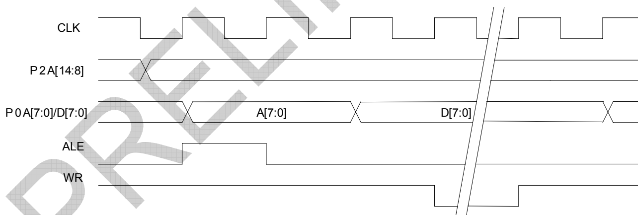
FIGURE 38: DATA MEMORY WRITE CYCLE TIMING
