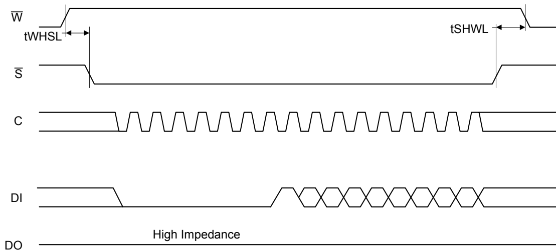
Figure 30. Write Protect Setup and Hold Timing during WRSR when (SRP1, SRP0) = (0, 1)
