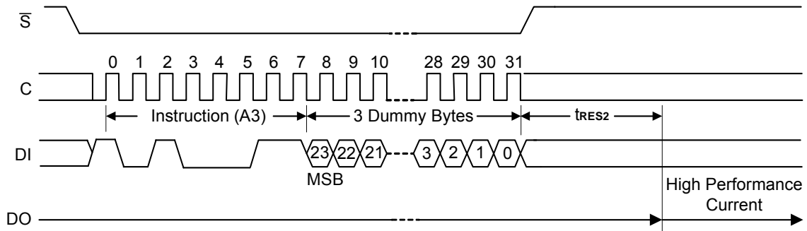
Figure 25. High Performance Mode Instruction Sequence
