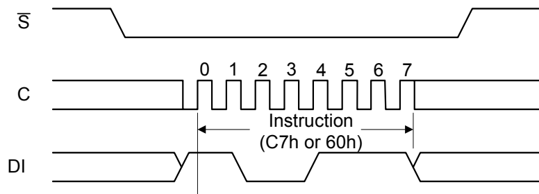
Figure 19. Chip Erase (CE) Instruction Sequence
