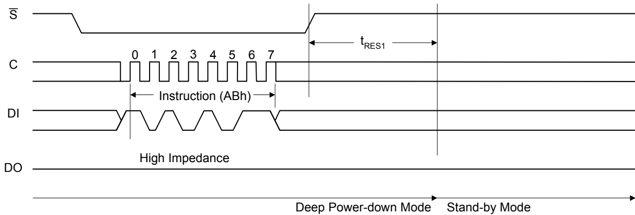
Figure 24. Release from Deep Power-down (RES) Instruction Sequence
