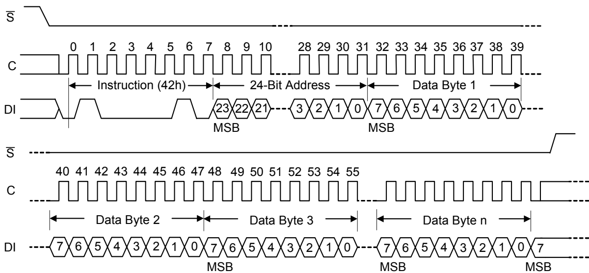
Figure 13. Program OTP (POTP) instruction sequence
