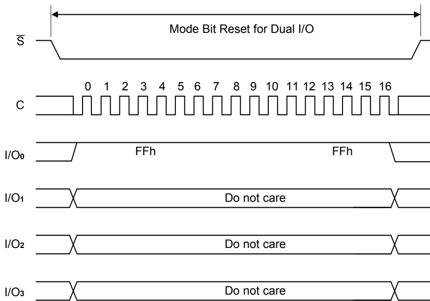
Figure 26. Continuous Read Mode Reset for Fast Read Dual I/O
