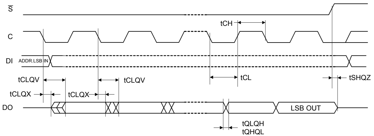
Figure 32. Output Timing
