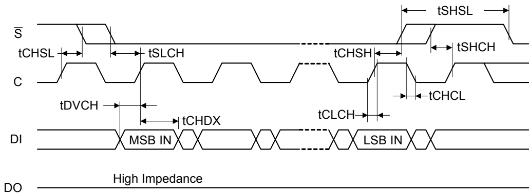
Figure 29. Serial Input Timing
