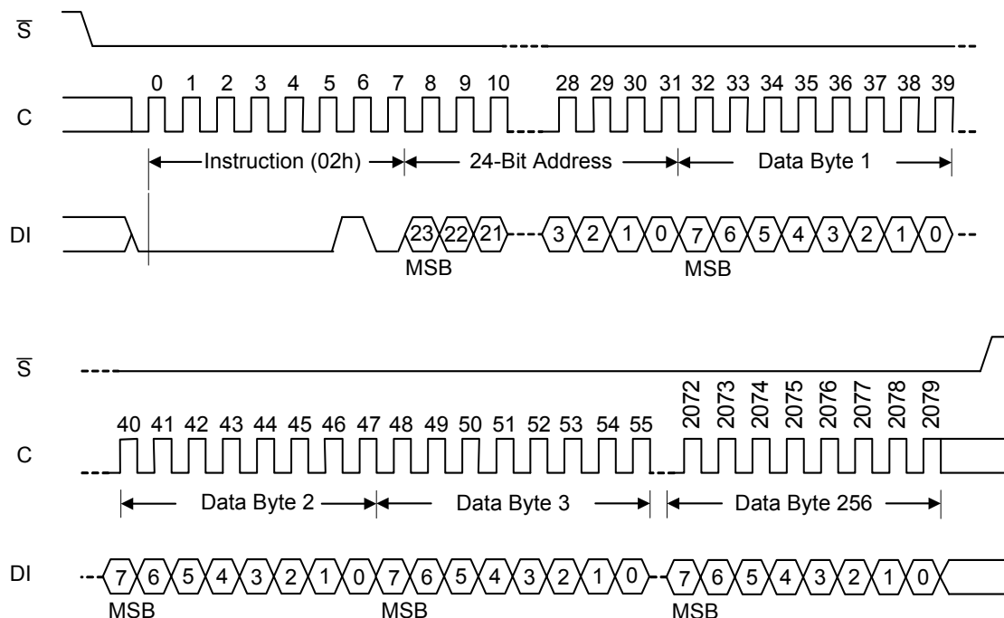
Figure 15. Page Program (PP) Instruction Sequence
