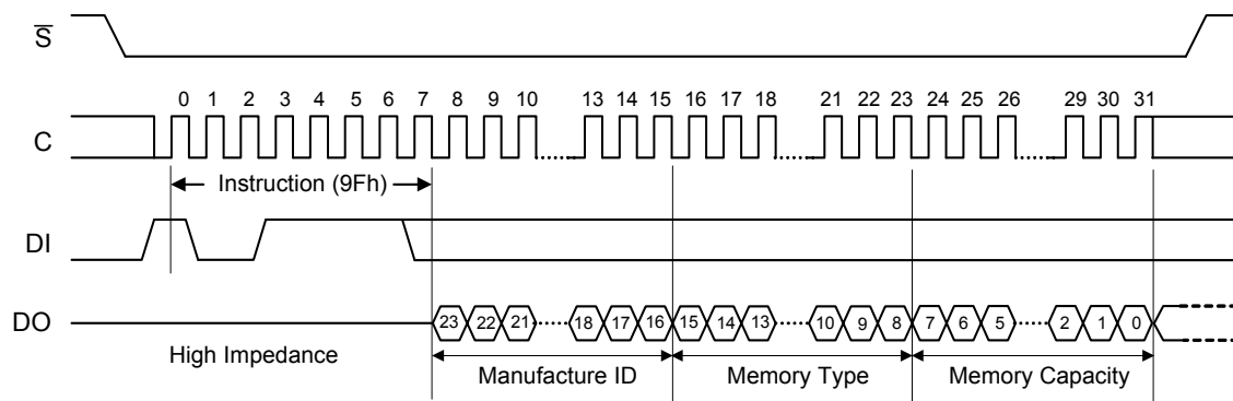
Figure 21. Read Identification (RDID) Instruction Sequence and Data-Out Sequence
