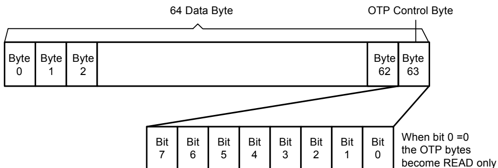
Figure 14. How to permanently lock the 64 OTP bytes
