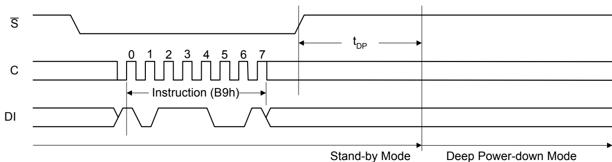
Figure 20. Deep Power-down (DP) Instruction Sequence
