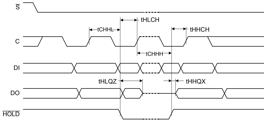
Figure 31. Hold Timing
