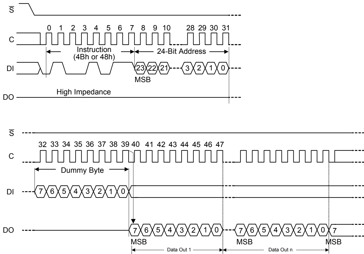
Figure 12. Read OTP (ROTP) instruction and data-out sequence
