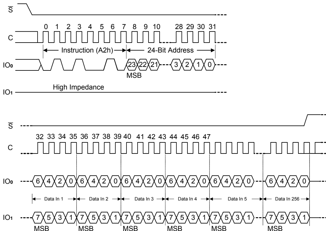
Figure 16. Dual Input Fast Program (DIFP) instruction sequence
