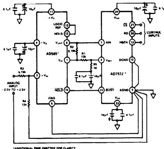
Figure 24. AD7572 - AD585 Sample-and-Hold Interface
