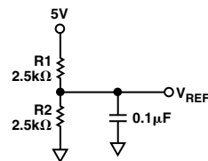
Figure 7. Midsupply Reference
