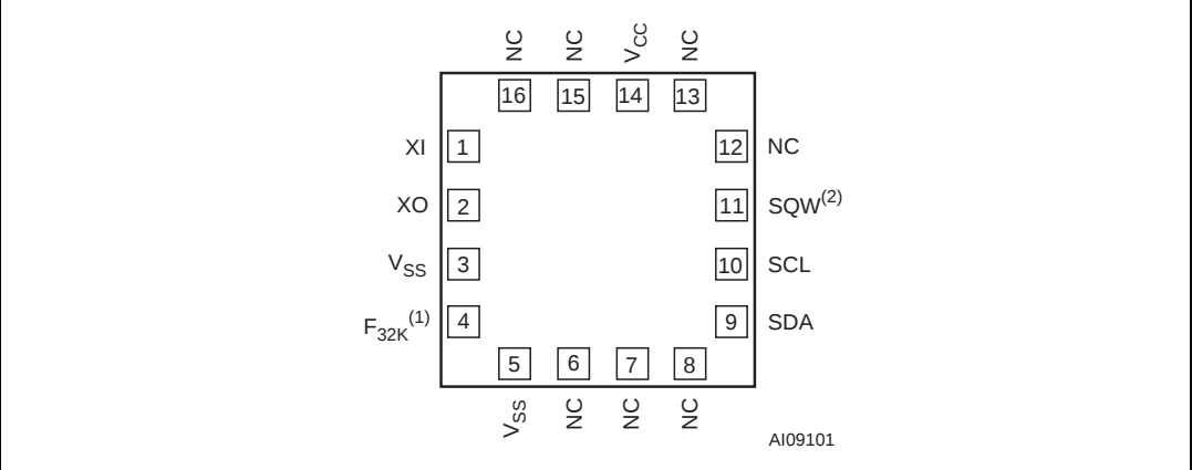
Figure 7. M41T64 connections
