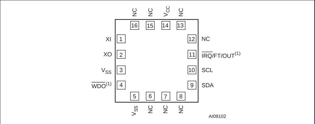
Figure 8. M41T65 connections
