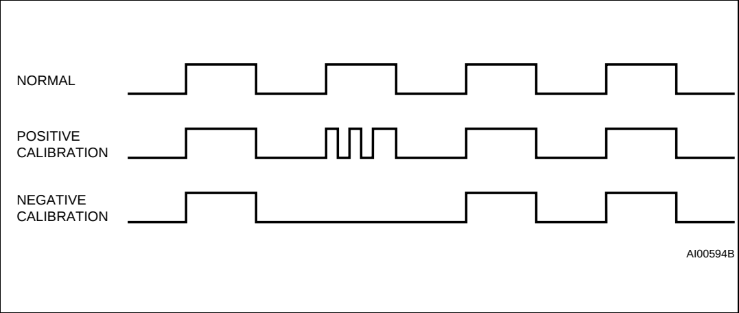
Figure 21. Calibration waveform
