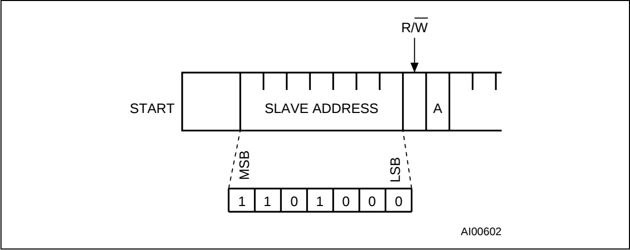
Figure 17. READ mode sequence
