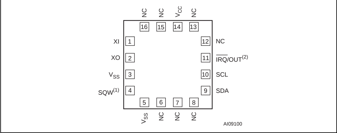
Figure 5. M41T62 connections
