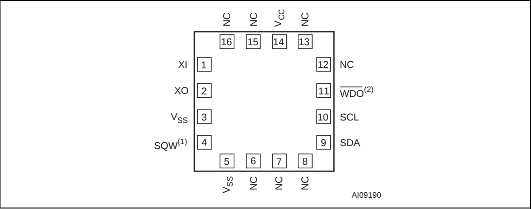
Figure 6. M41T63 connections
