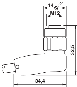
M12 x 1 socket, angled
