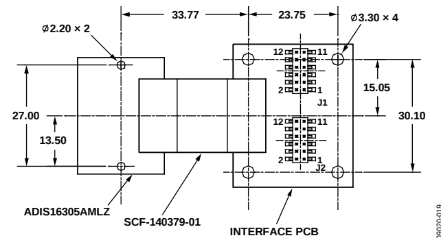
Figure 19. Physical Diagram for Mounting the ADIS16305/PCBZ
