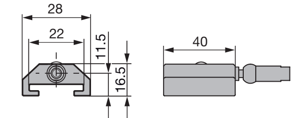
Fig. 11-6: Installation dimensions of BTL5-T-2814-1S magnet
