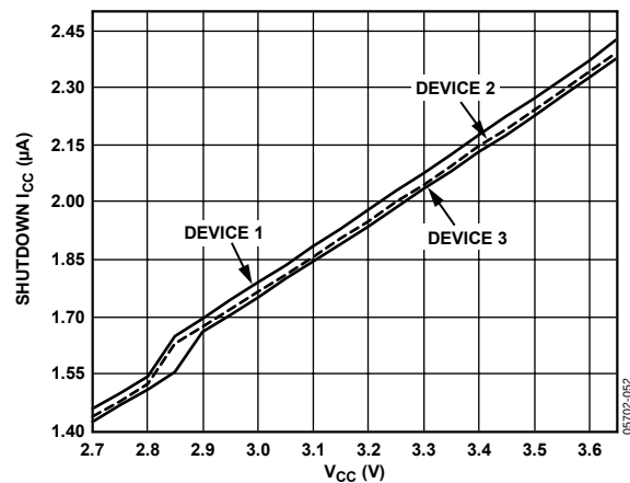
Figure 11. Shutdown Supply Current vs. Supply Voltage ( V_{CC} = AV_{CC} + DV_{CC} , I_{CC} = AI_{CC} + DI_{CC} )
