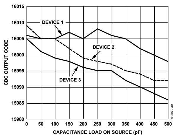
Figure 13. Output Code vs. Capacitive Load on SRC
