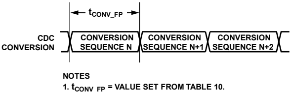
Figure 26. Full Power Mode CDC Conversion Sequence Time
