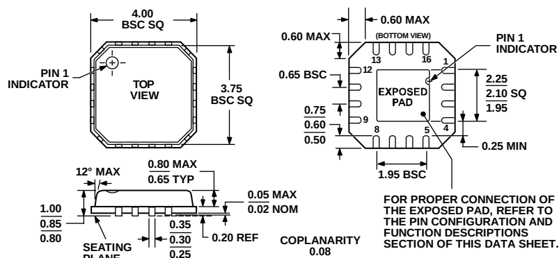
Figure 23. 16-Lead Lead Frame Chip Scale Package [LFCSP_VQ] 4 mm × 4 mm Body, Very Thin Quad (CP-16-4)
