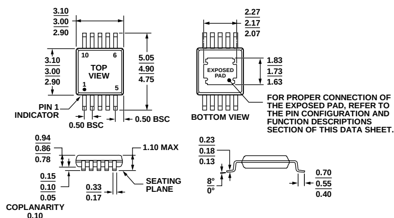
Figure 22. 10-Lead Mini Small Outline Package with Exposed Pad [MINI_SO_EP] (RH-10-1)
