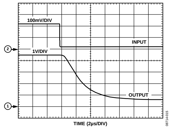
Figure 15. Fall Time
