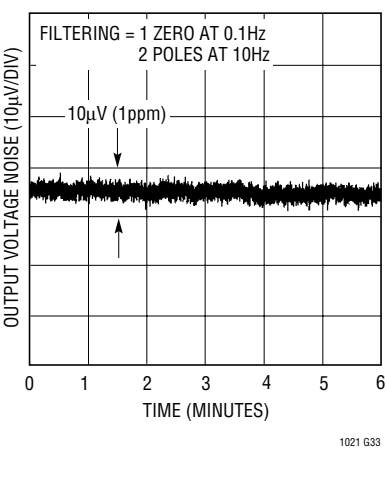
Output Noise 0.1Hz to 10Hz LT1021-10
