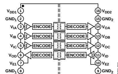
Figure 2. ADuM1401
