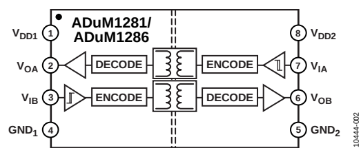
Figure 2. ADuM1281/ADuM1286
