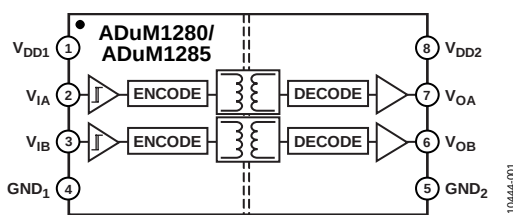
Figure 1. ADuM1280/ADuM1285
