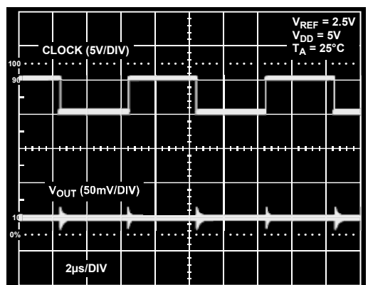
Figure 18. Digital Feedthrough
