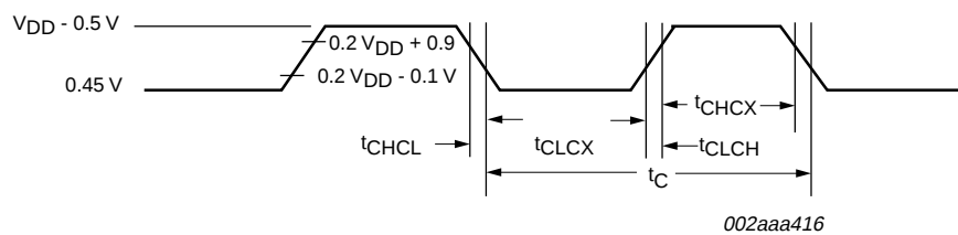
Fig 22. External clock timing.
