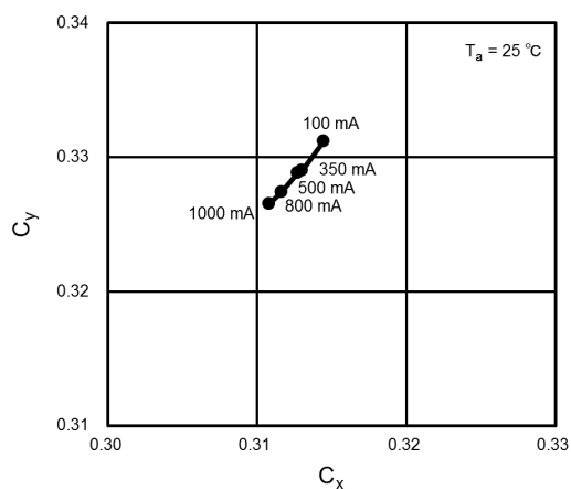
Fig. 8.4 Chromaticity - I_F
