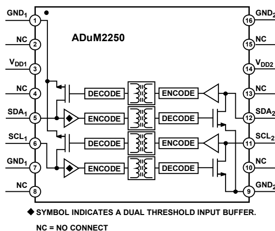
Figure 6. ADuM2250 Block Diagram
