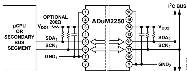
Figure 7. Typical Isolated I 2 C Interface Using ADuM2250
