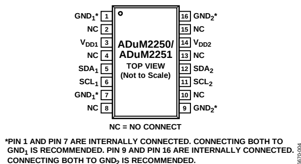
Figure 5. Pin Configuration
