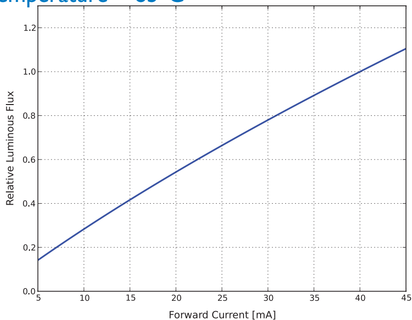
Figure 6. Typical relative luminous flux vs. forward current, LXAC-I827 and LXAC-I830.
