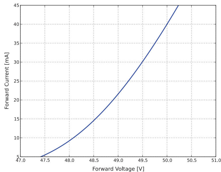
Figure 7. Typical forward current vs. forward voltage, LXAC-I827 and LXAC-I830.
