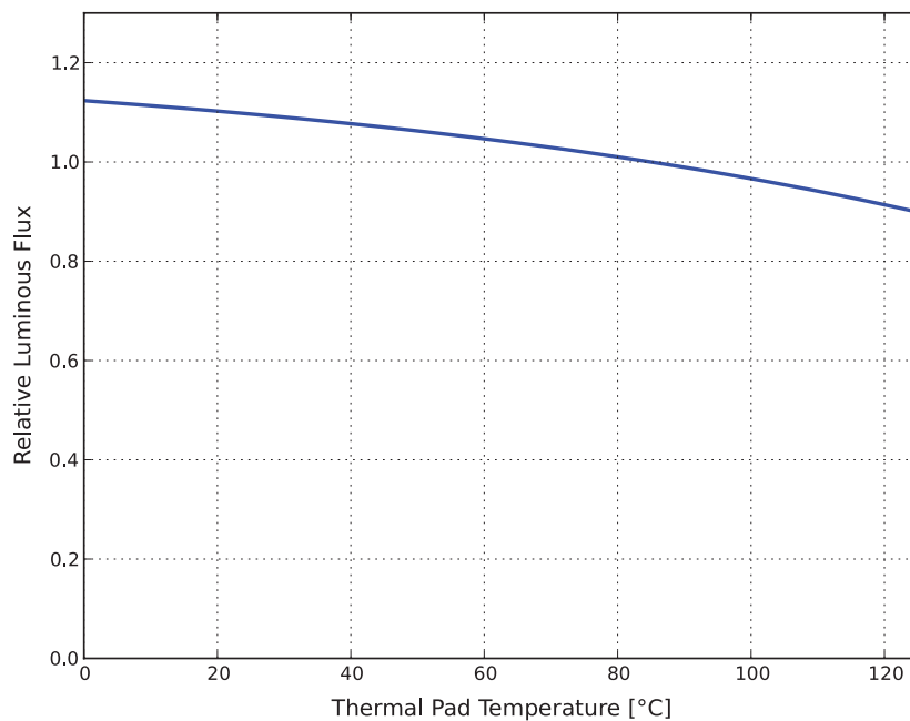
Figure 5. Relative light output vs. thermal pad temperature, LXAC-I827 and LXAC-I830.
