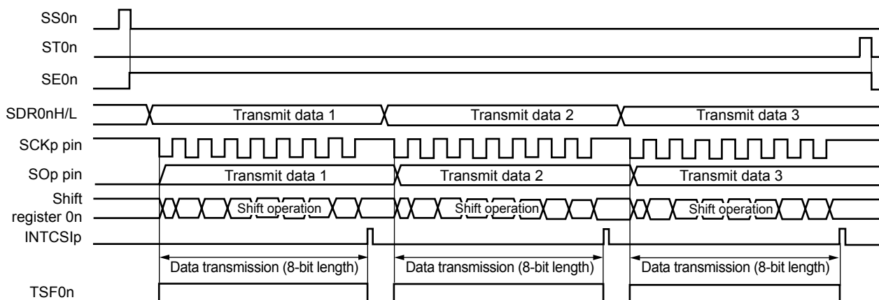
Figure 10-28. Timing Chart of Master Transmission (in Single-Transmission Mode) (Type 1: DAP0n = 0, CKP0n = 0)
