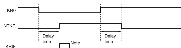
Figure 12-6. Operation of INTKR Signal When a Key Interrupt is Input to a Single Channel (When KRMD = 0 and KREG = 0)
