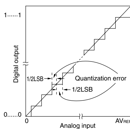
Figure 9-17. Quantization Error
