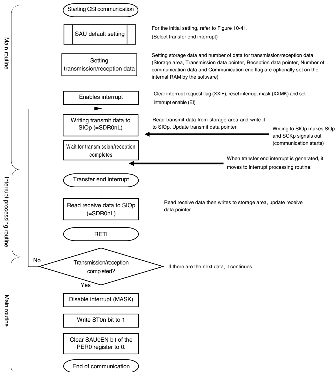
Figure 10-45. Flowchart of Master Transmission/Reception (in Single-Transmission/Reception Mode)
