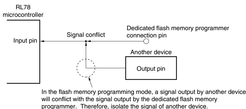
Figure 17-5. Signal Conflict (RESET Pin)
