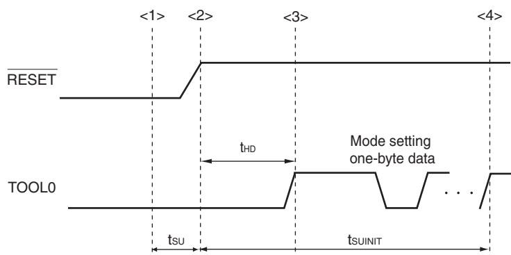
Figure 17-7. Entry to Flash Memory Programming Mode
