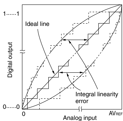
Figure 9-20. Integral Linearity Error
