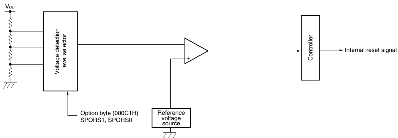
Figure 15-1. Block Diagram of Selectable Power-on-reset Circuit
