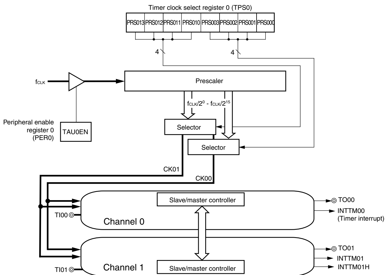
Figure 6-1. Entire Configuration of Timer Array Unit
