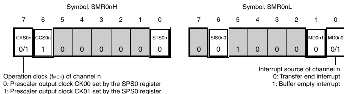
Figure 10-48. Example of Contents of Registers for Slave Transmission of 3-Wire Serial I/O (CSI00) (1/2)
