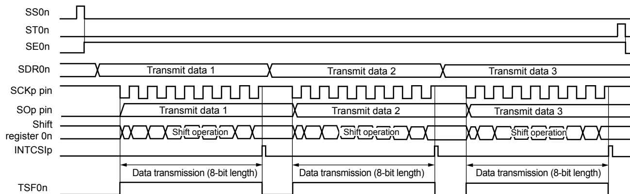
Figure 10-52. Timing Chart of Slave Transmission (in Single-Transmission Mode)
