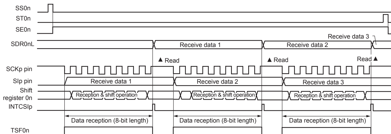
Figure 10-60. Timing Chart of Slave Reception (in Single-Reception Mode)
