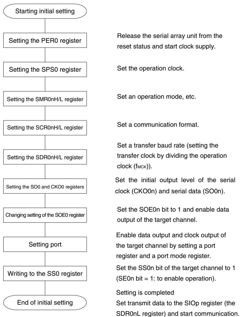
Figure 10-41. Initial Setting Procedure for Master Transmission/Reception
