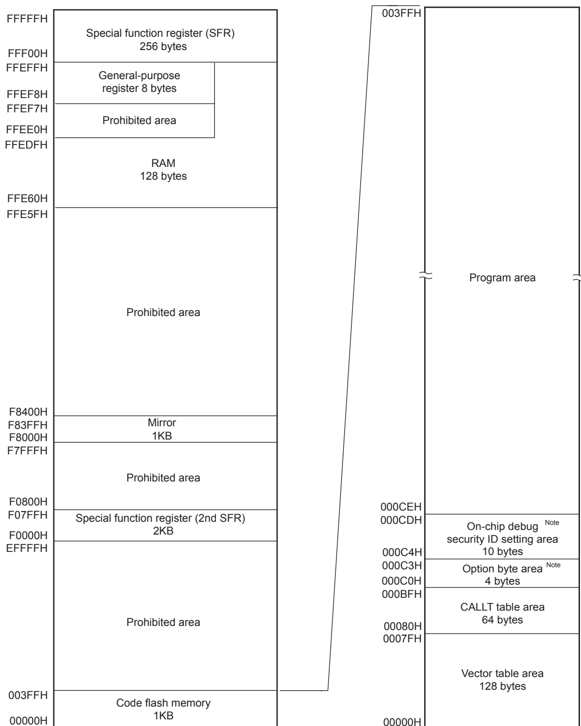
Figure 3-1. Memory Map for the R7F0C80112ESP
