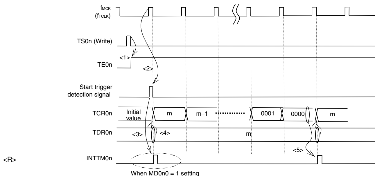
Figure 6-24. Operation Timing (In Interval Timer Mode)
