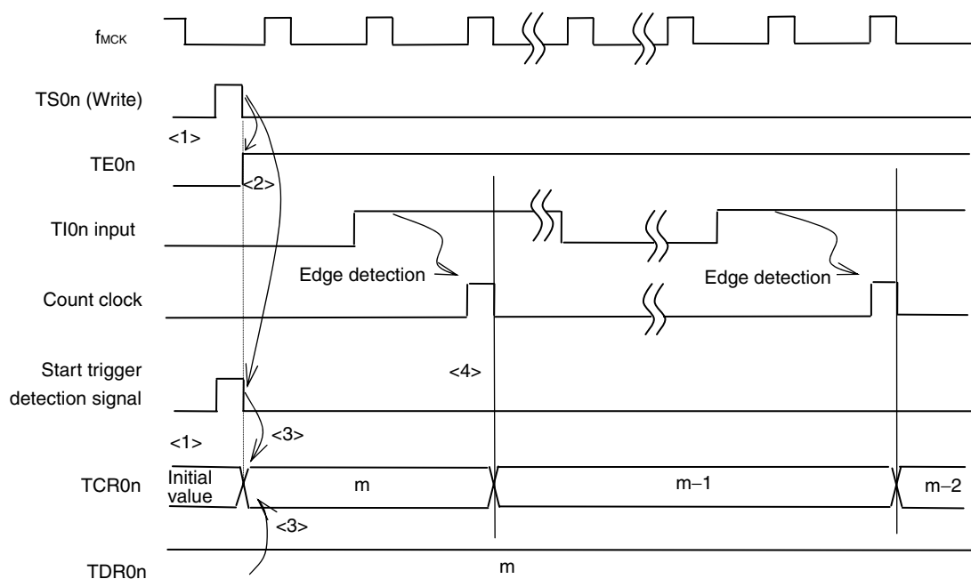
Figure 6-25. Operation Timing (In Event Counter Mode)
