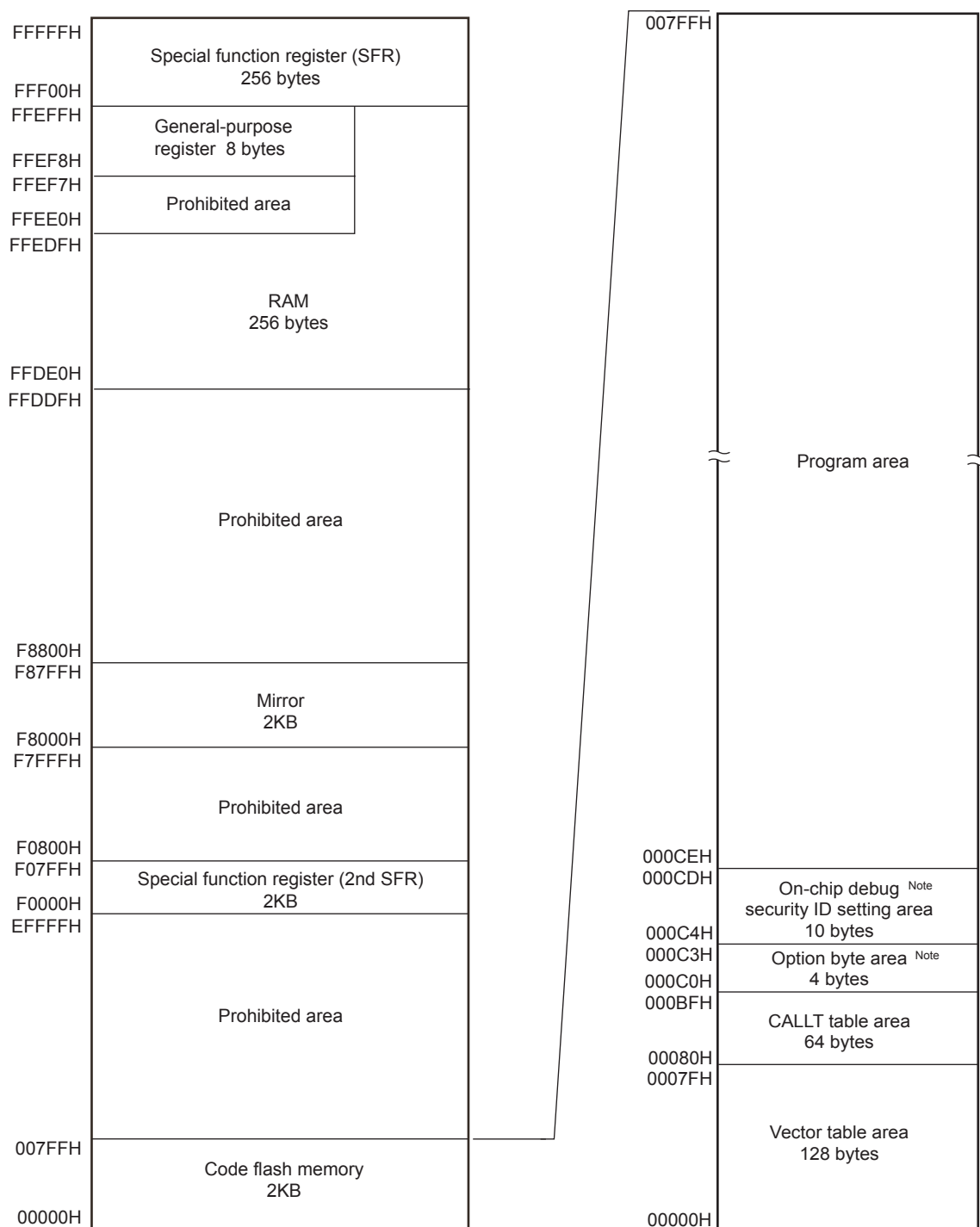
Figure 3-2. Memory Map for the R7F0C80212ESP
