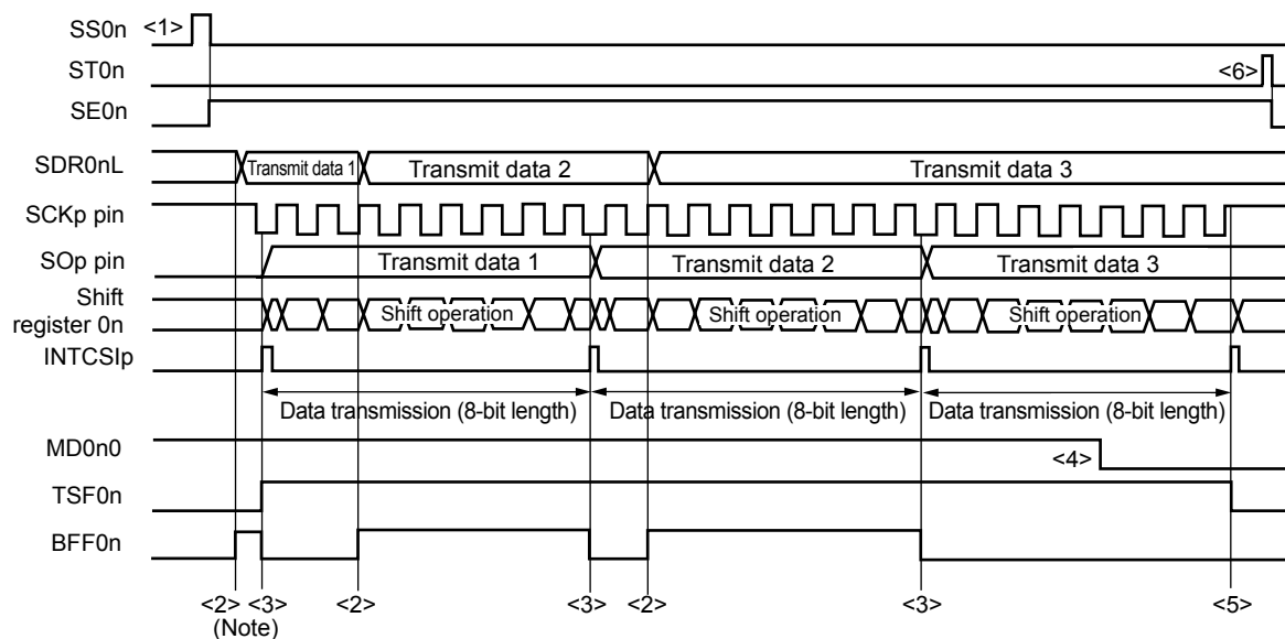
Figure 10-54. Timing Chart of Slave Transmission (in Continuous Transmission Mode)
