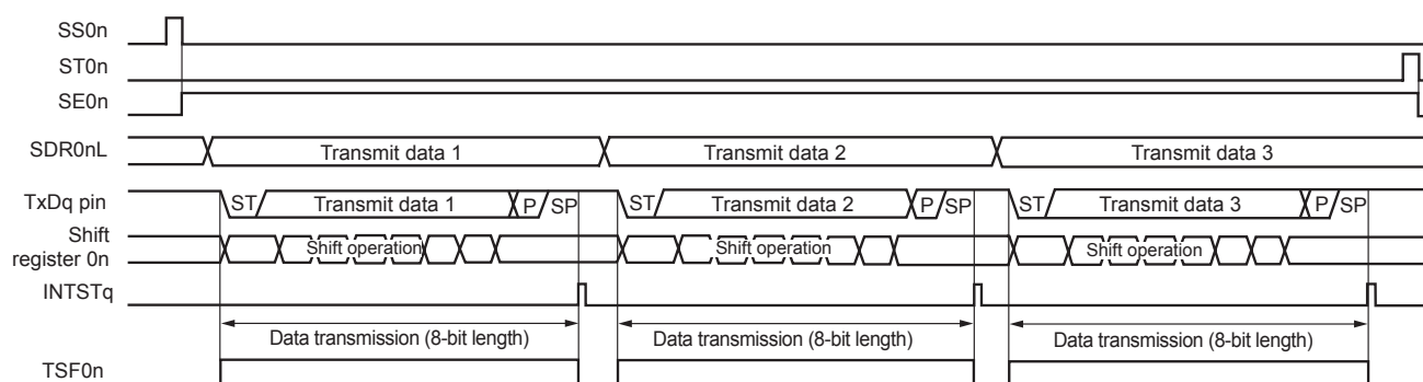
Figure 10-75. Timing Chart of UART Transmission (in Single-Transmission Mode)
