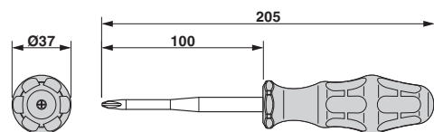
Dimensioned drawing
