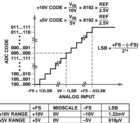
Figure 35. Transfer Characteristics
