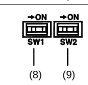
DIP switch for Units with 10/20 I/O points
