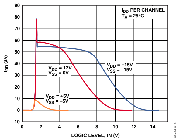
Figure 13. I_{DD} vs. Logic Level
